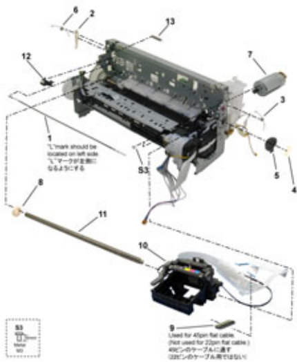
FIGURE 9 PURGE UNIT
