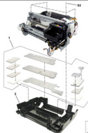
FIGURE 6 SHEET FEED UNIT
