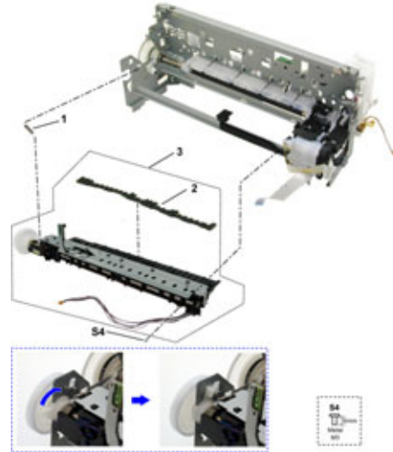
FIGURE 8 PLATEN UNIT
