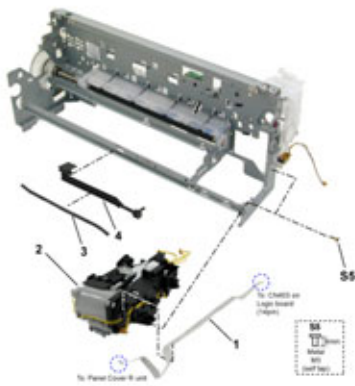
FIGURE 9 PURGE UNIT
