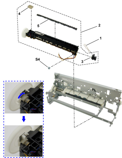
FIGURE 12 PAPER FEED & CARRIAGE LIFT PART (PIXMA iP4000/PIXUS iP4100)
