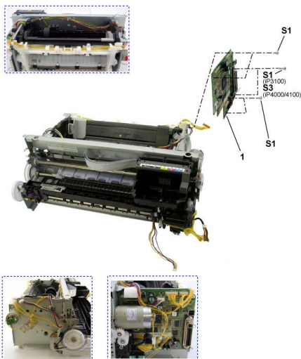
FIGURE 5 LOGIC BOARD
