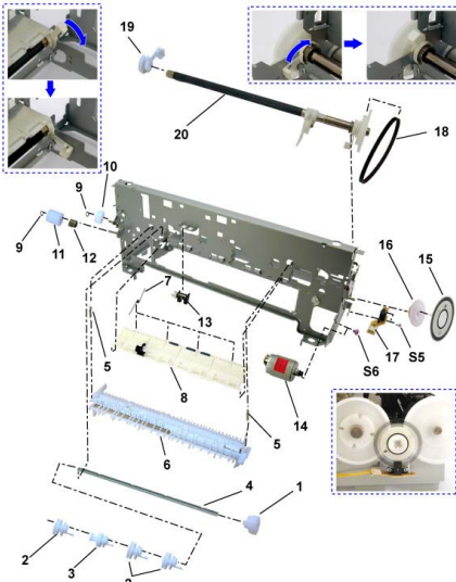
FIGURE 11 PAPER FEED & CARRIAGE LIFT PART (PIXUS iP3100)
