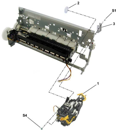
FIGURE 11 PAPER FEED & CARRIAGE LIFT PART (PIXUS iP3100)
