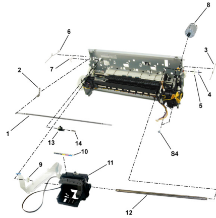
FIGURE 8 CARRIAGE UNIT
