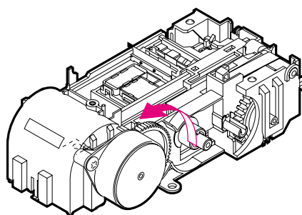
Purge Unit
