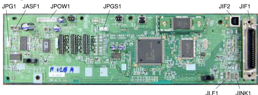
Figure 4-4 Logic Board
