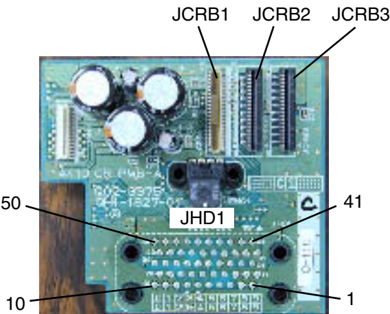
Figure 4-2 Carriage Board
