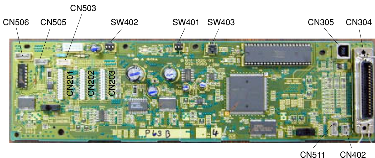
Figure 4-10 Logic Board
