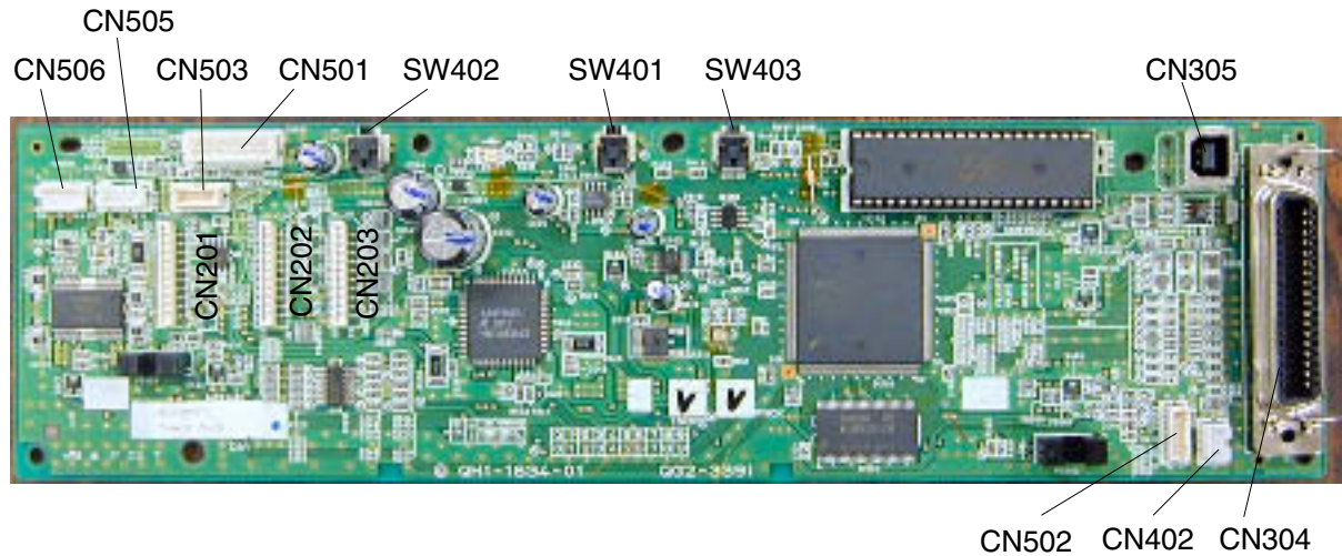
Figure 4-7 Logic Board
