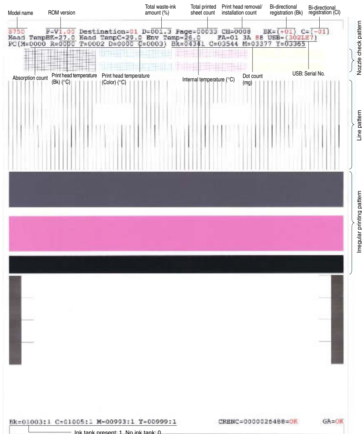
Figure 2-13 Service/Factory Test Printout (Sample)
