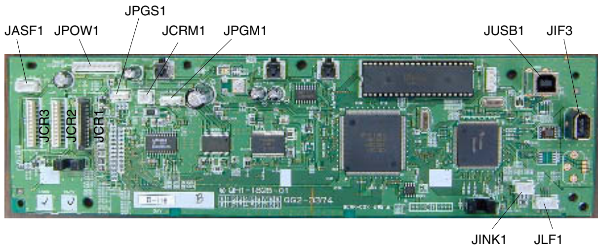
Figure 4-1 Logic Board
