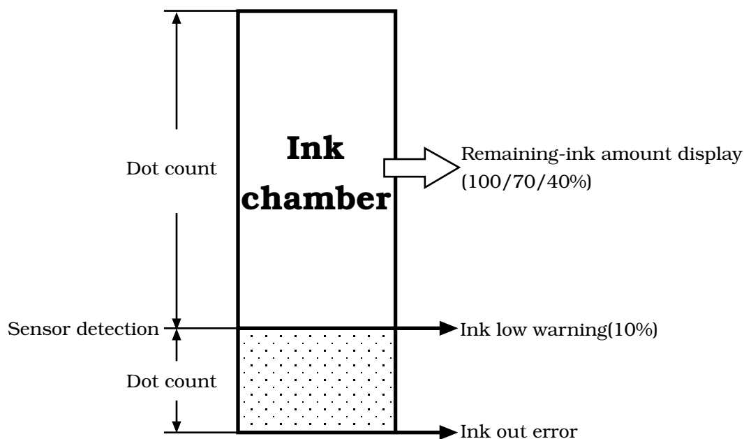
Figure 3-1 Remaining-ink amount detection
