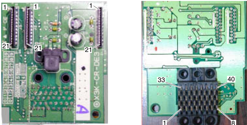
Figure 4-8 Carriage Board
