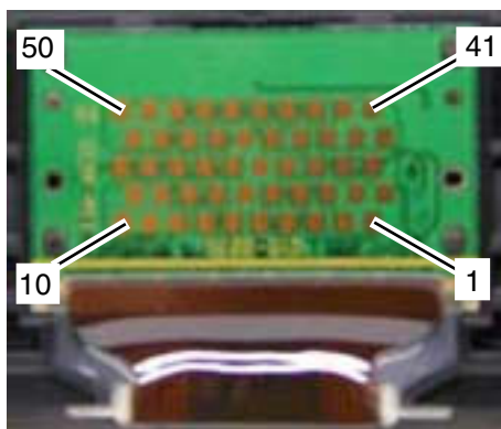
Figure 4-3 Print Head
