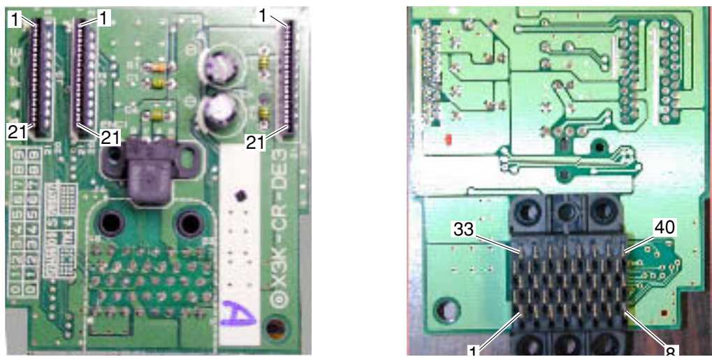
Figure 4-11 Carriage Board
