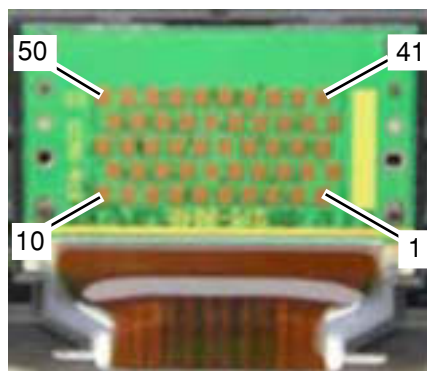
Figure 4-6 Print Head
