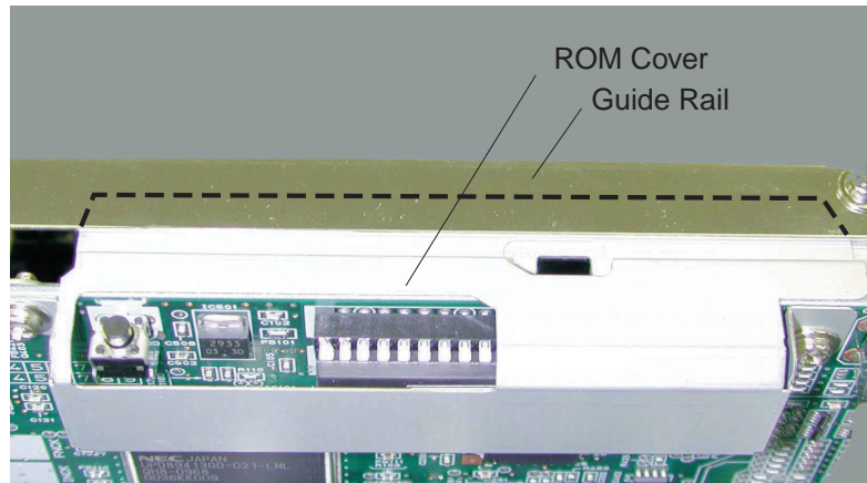
Figure 2-10 Installing the ROM Cover
