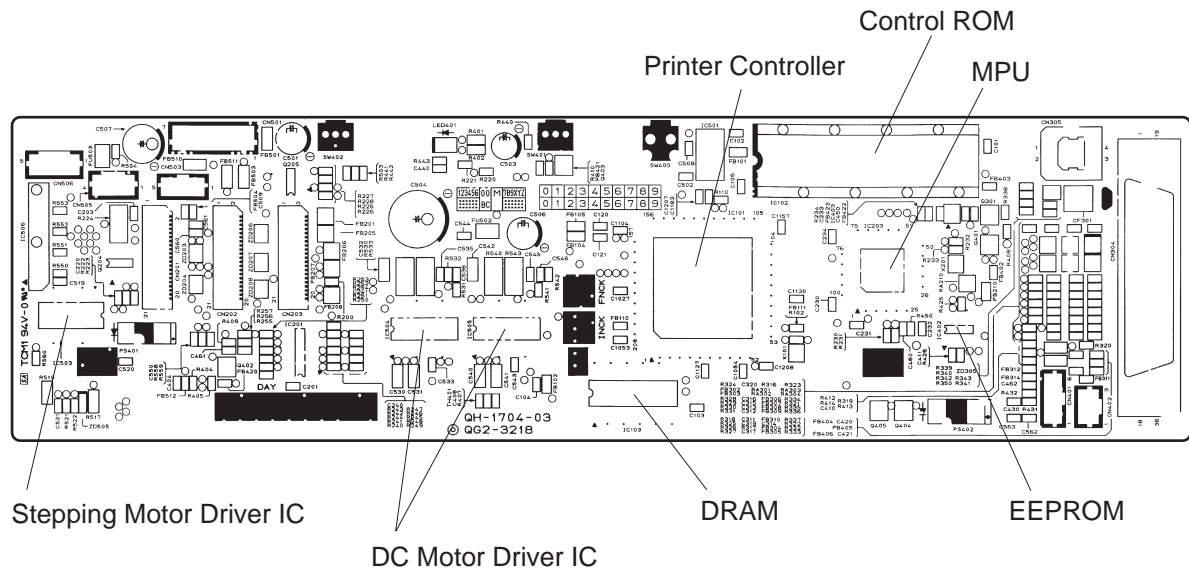
Figure 3-12 Control Board
