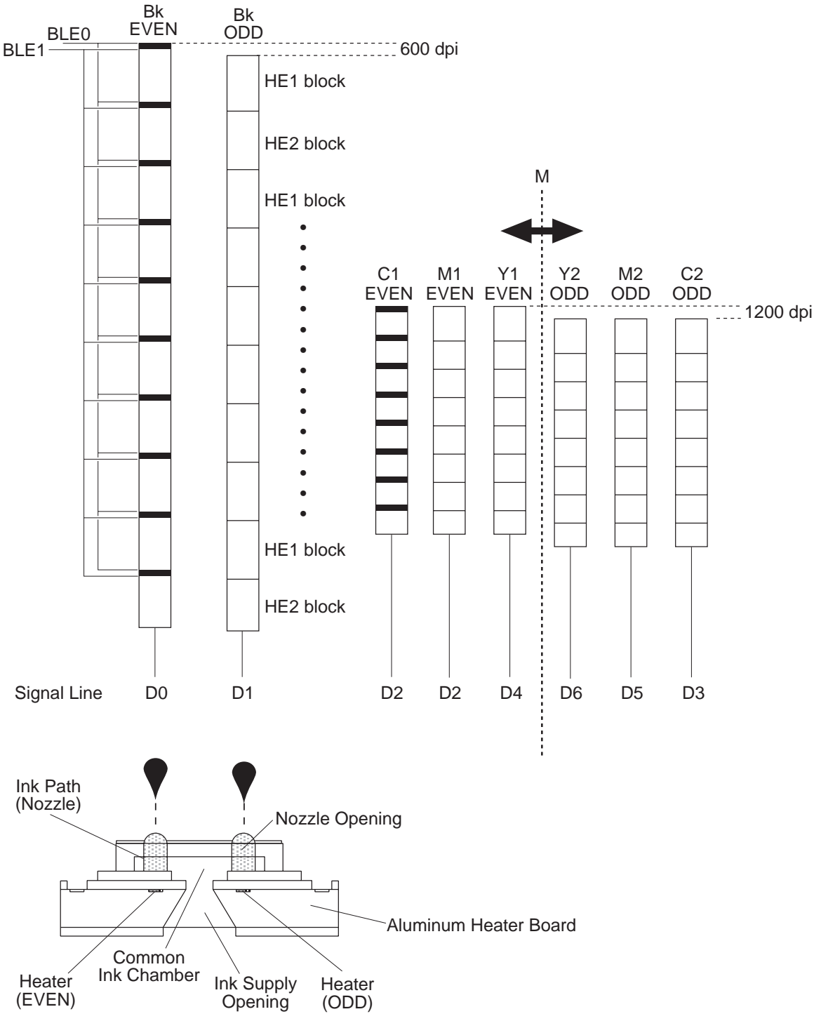
Figure 3-14 Nozzle Array
