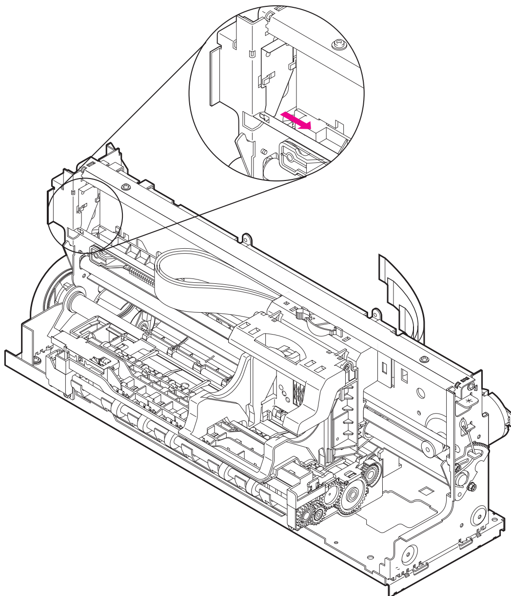
Figure 2-5 Encoder Film
