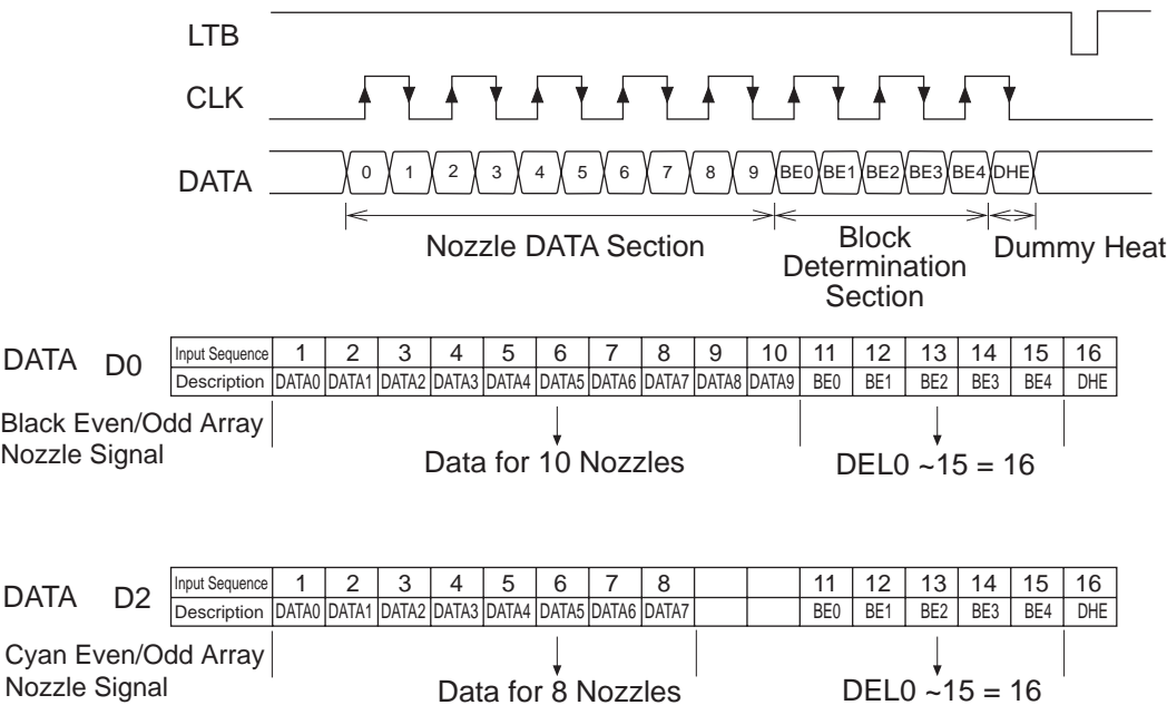
Figure 3-2 Serial Data
