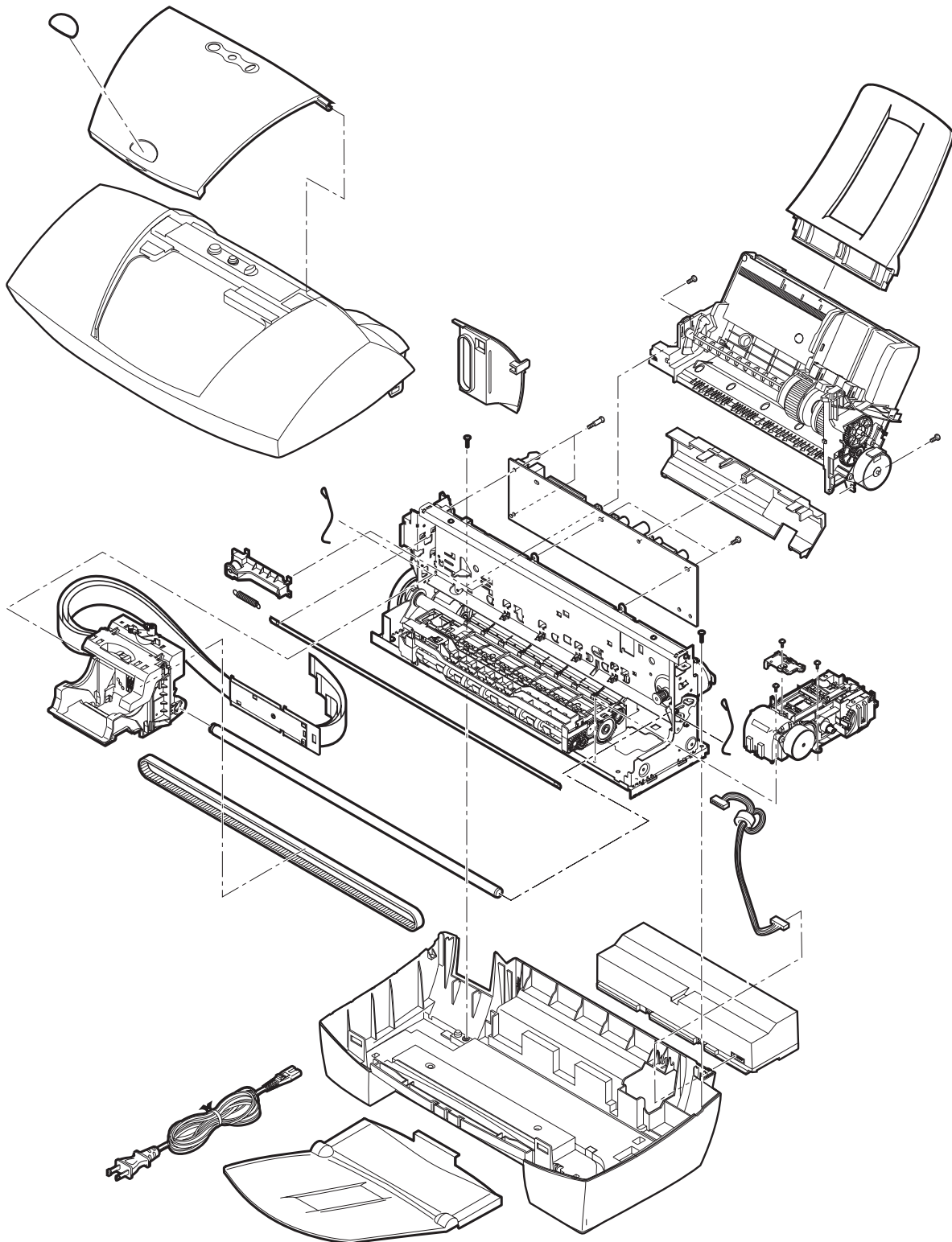
Figure 2-3 Exploded View
