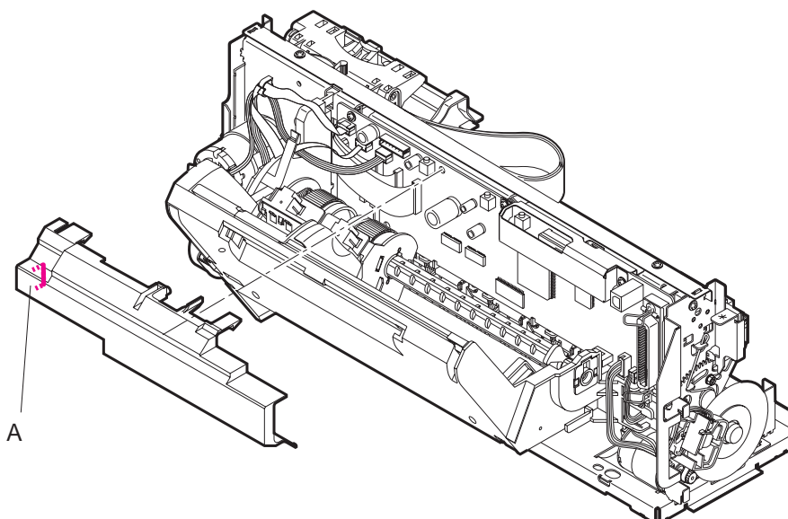
Figure 2-8 Installing the Logic Board Cover
