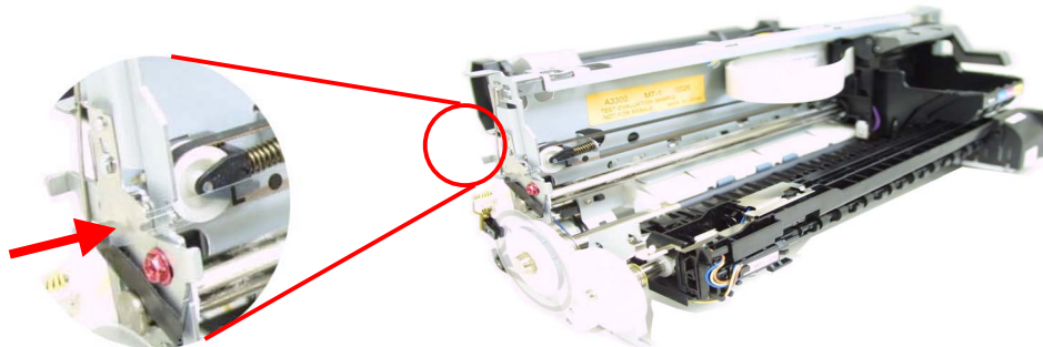
Figure 1-2 Code Strip
