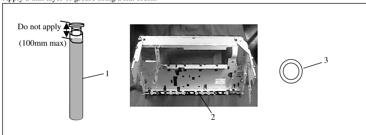
Figure 1-4 Applying Grease
