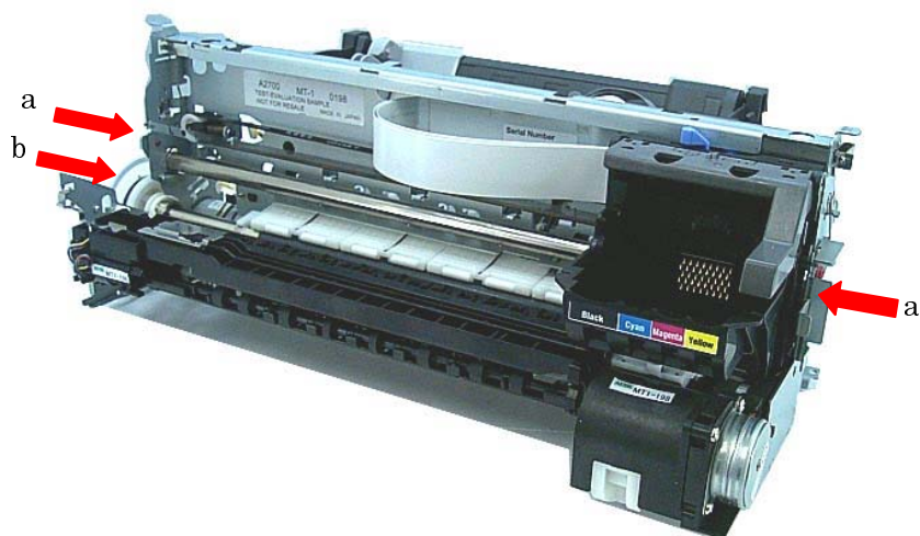
Figure 1-3 Do Not Loosen or Remove Red Screws
