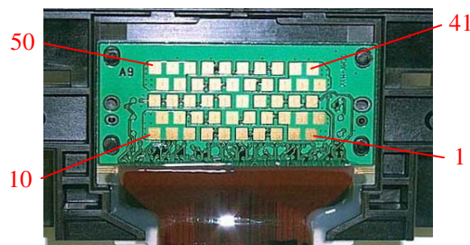
Figure 3-9 Print Head
