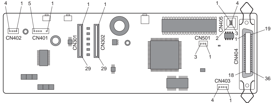
Figure 5-12 Control Board
