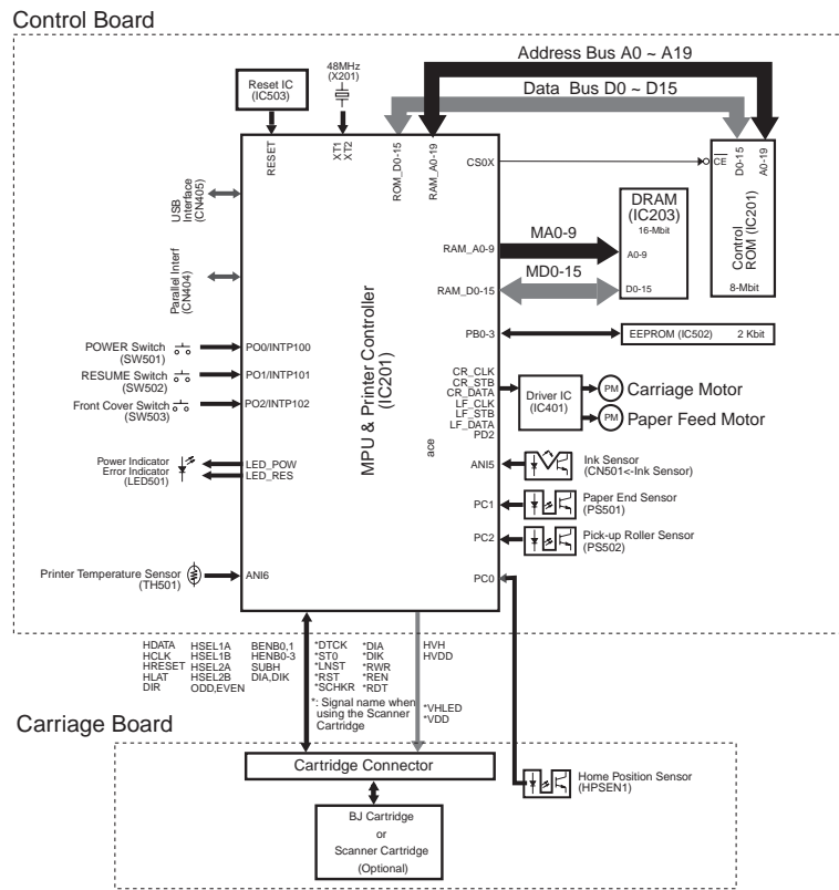
Figure 5-5 Block Diagram
