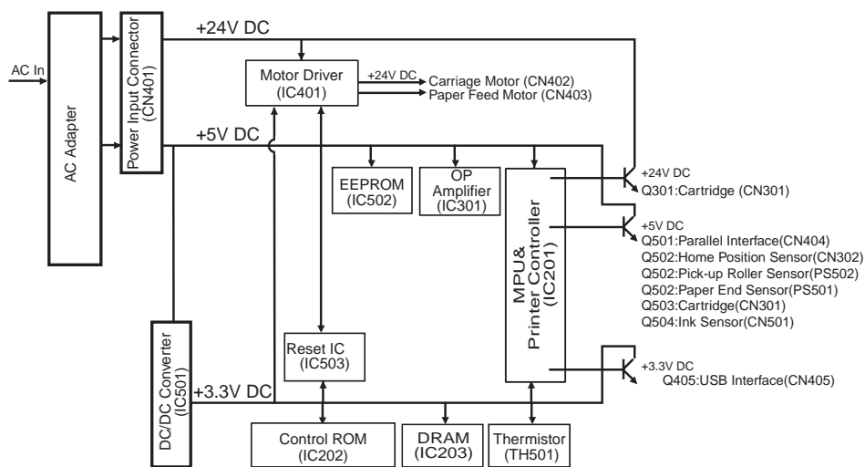
Figure 5-6 Power Line Block Diagram
