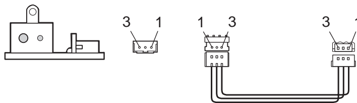
Figure 5-21 Ink Sensor
